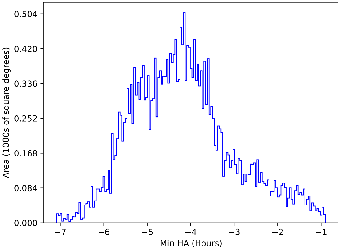
too_elab_r64_d3_griz_v3.4_10yrs All sky r band: Min HA
