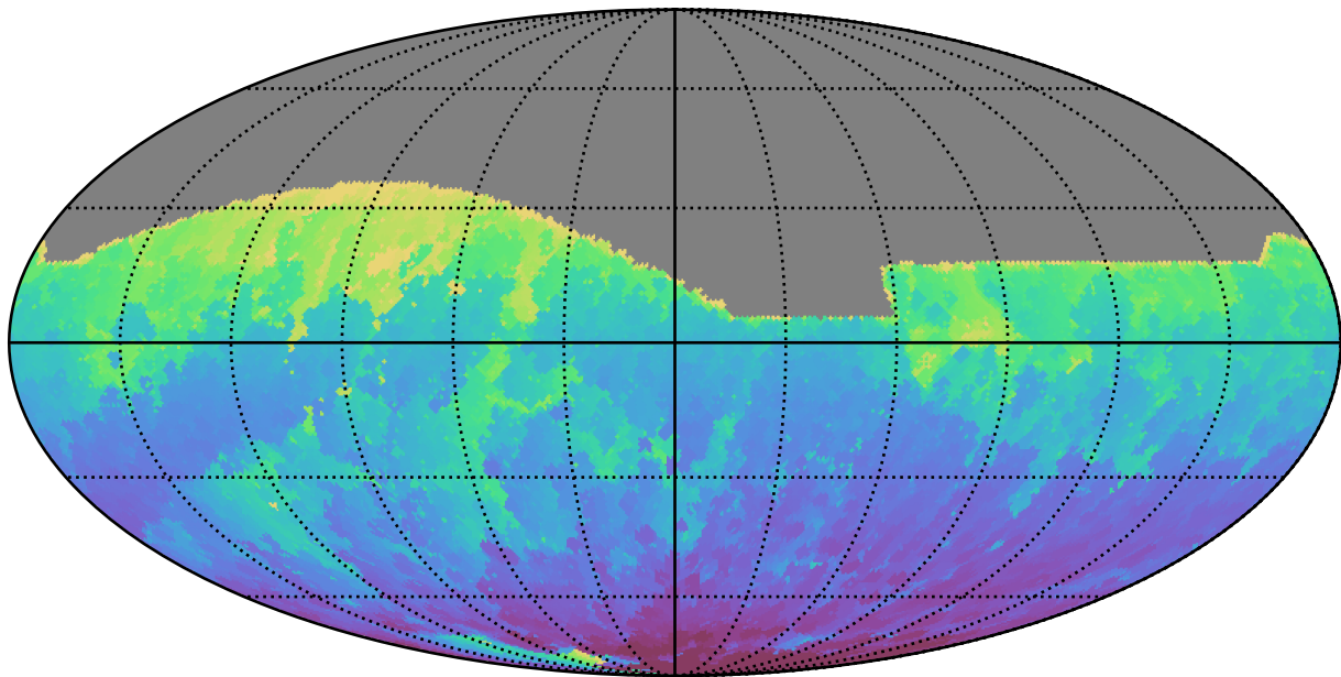
too_elab_r64_d3_griz_v3.4_10yrs All sky i band: Min HA
