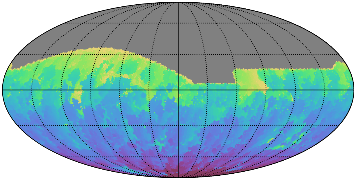
too_elab_r64_d3_griz_v3.4_10yrs All sky g band: Min HA
