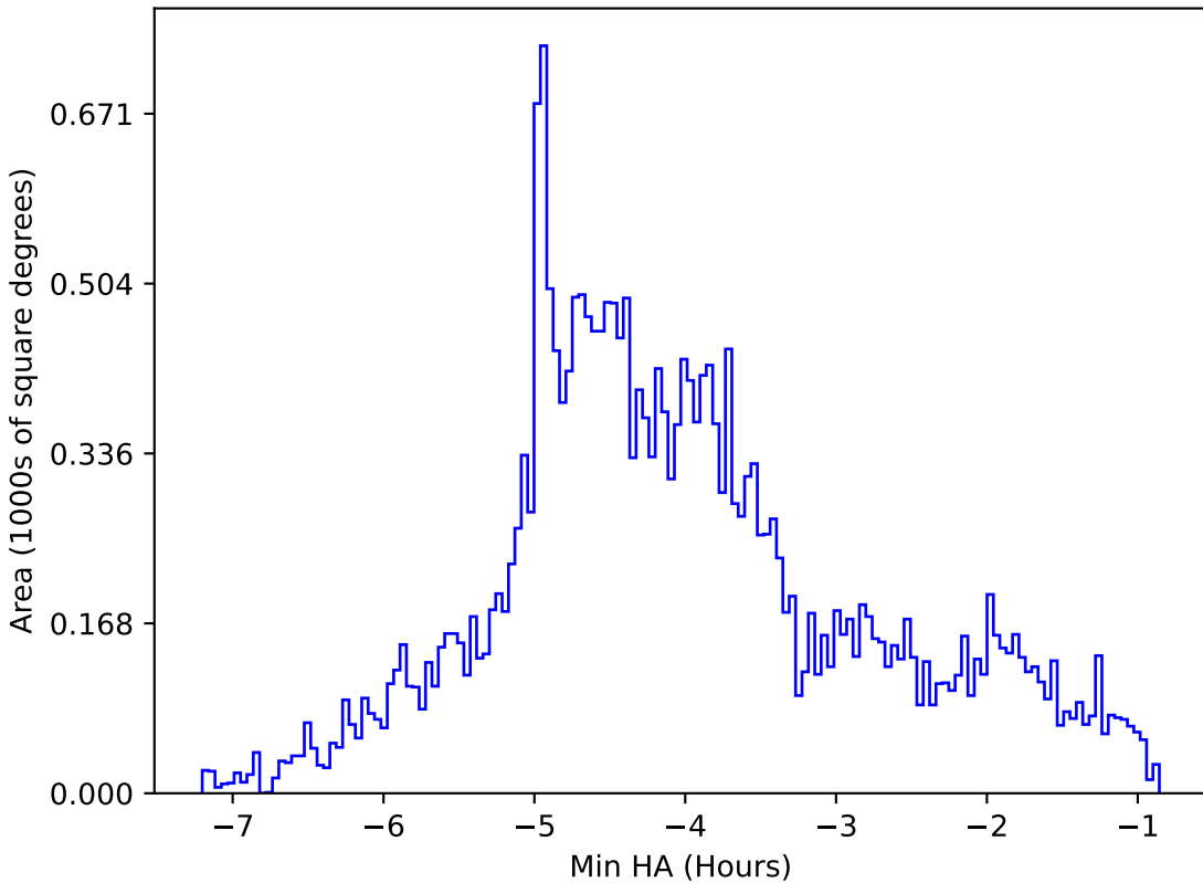
too_elab_r64_d3_griz_v3.4_10yrs All sky g band: Min HA
