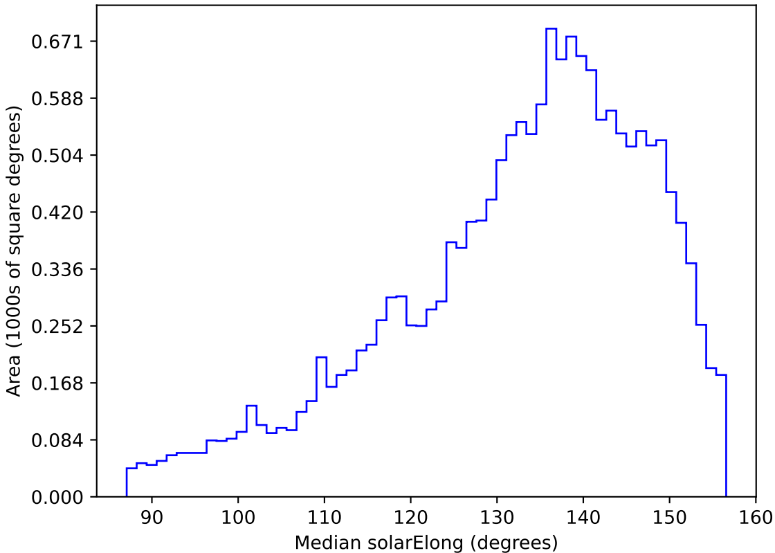
too_elab_r64_d3_griz_v3.4_10yrs WFD u band: Median solarElong
