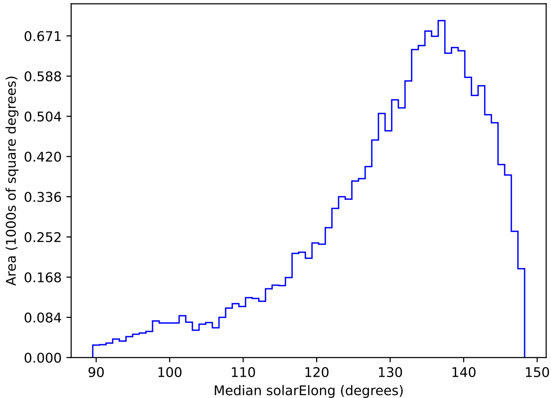
too_elab_r64_d3_griz_v3.4_10yrs WFD r band: Median solarElong
