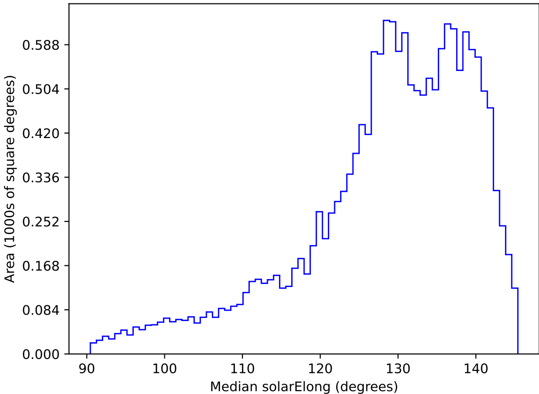
too_elab_r64_d3_griz_v3.4_10yrs WFD i band: Median solarElong
