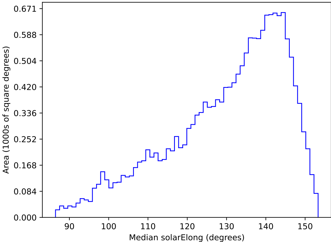
too_elab_r64_d3_griz_v3.4_10yrs WFD g band: Median solarElong
