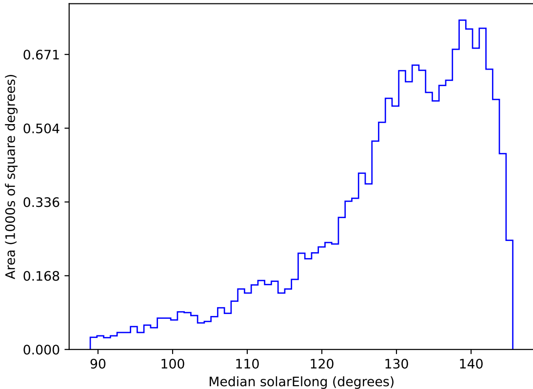
too_elab_r64_d3_griz_v3.4_10yrs WFD all bands: Median solarElong
