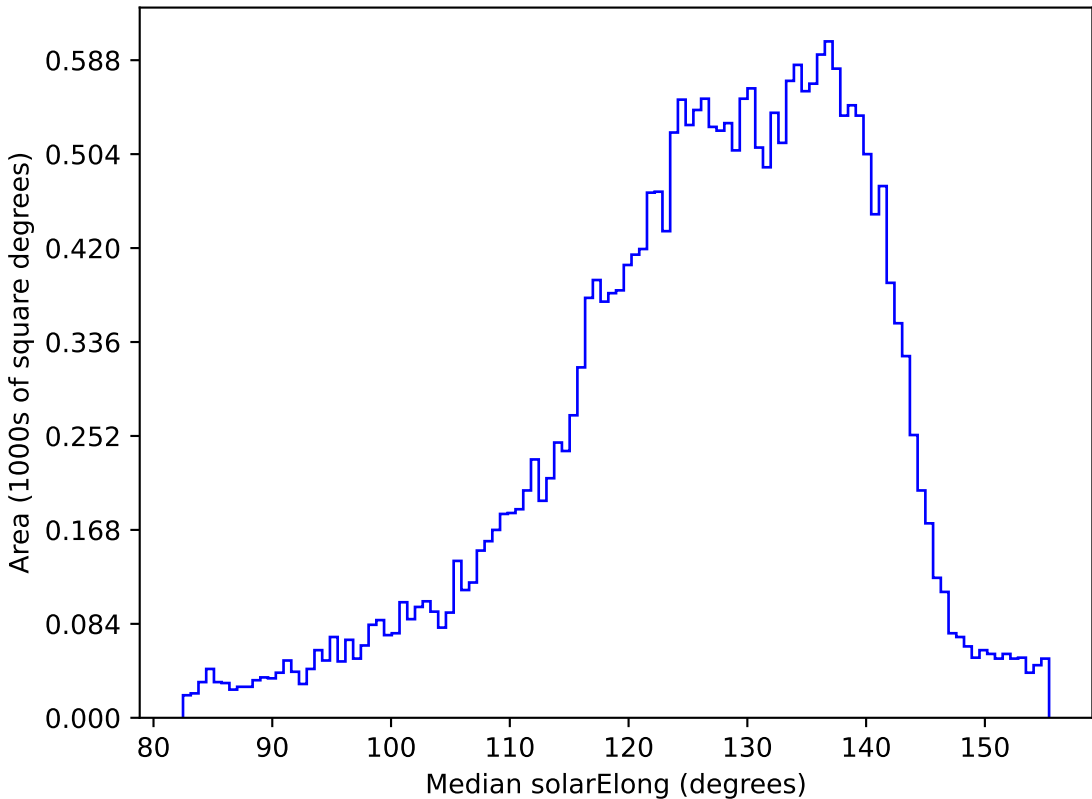
too_elab_r64_d3_griz_v3.4_10yrs All sky z band: Median solarElong
