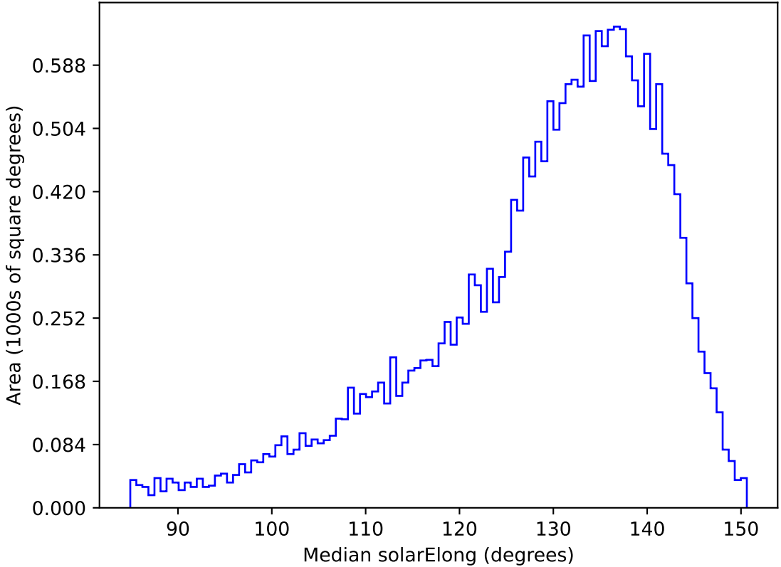
too_elab_r64_d3_griz_v3.4_10yrs All sky y band: Median solarElong
