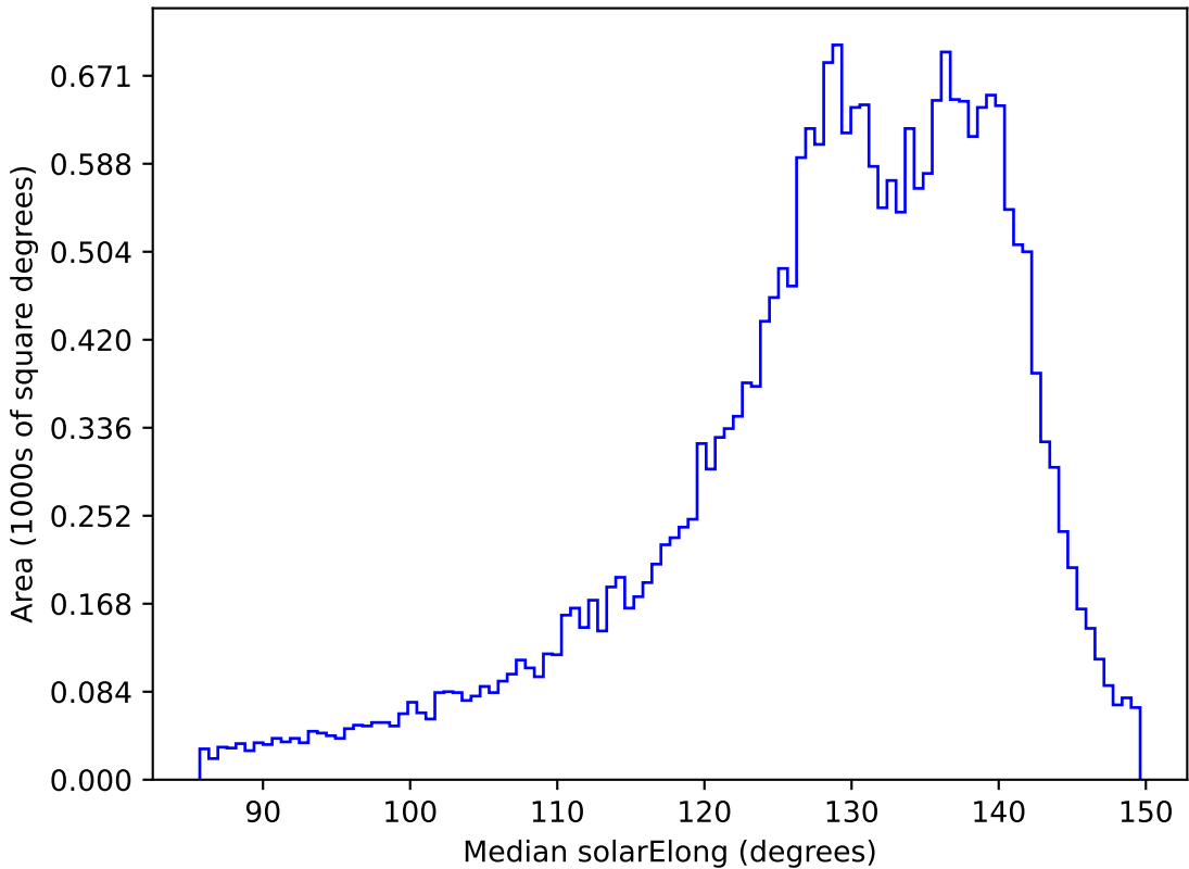
too_elab_r64_d3_griz_v3.4_10yrs All sky i band: Median solarElong
