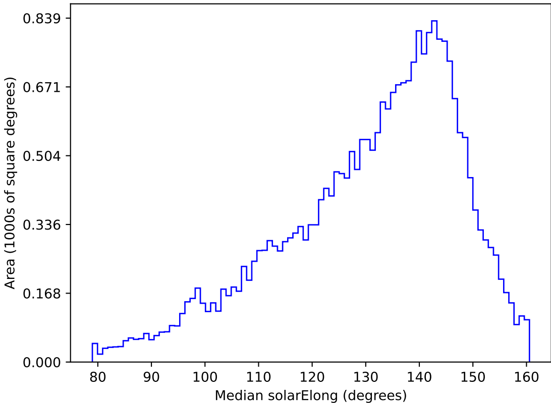
too_elab_r64_d3_griz_v3.4_10yrs All sky g band: Median solarElong
