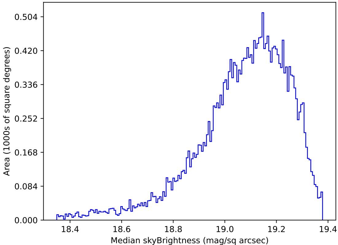
too_elab_r64_d3_griz_v3.4_10yrs Yr 1 z band: Median skyBrightness
