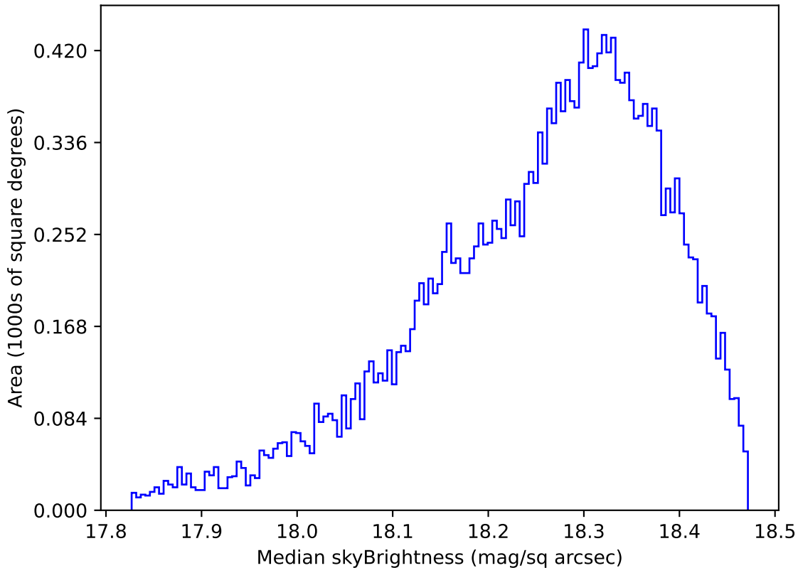
too_elab_r64_d3_griz_v3.4_10yrs Yr 1 y band: Median skyBrightness
