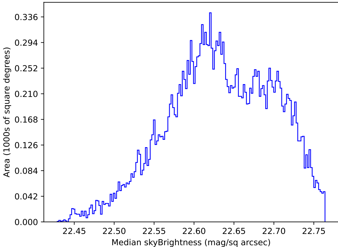
too_elab_r64_d3_griz_v3.4_10yrs Yr 1 u band: Median skyBrightness
