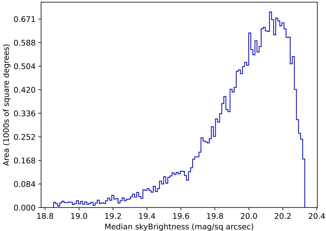
too_elab_r64_d3_griz_v3.4_10yrs Yr 1 i band: Median skyBrightness
