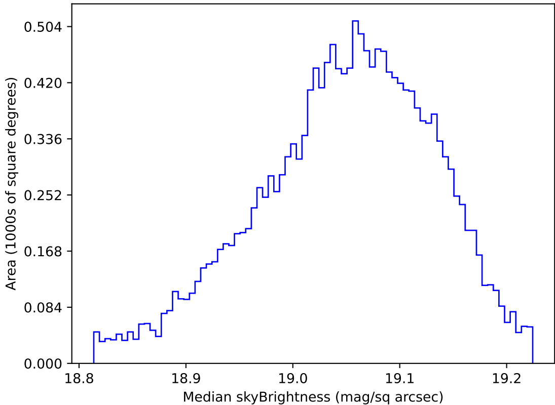
too_elab_r64_d3_griz_v3.4_10yrs WFD z band: Median skyBrightness
