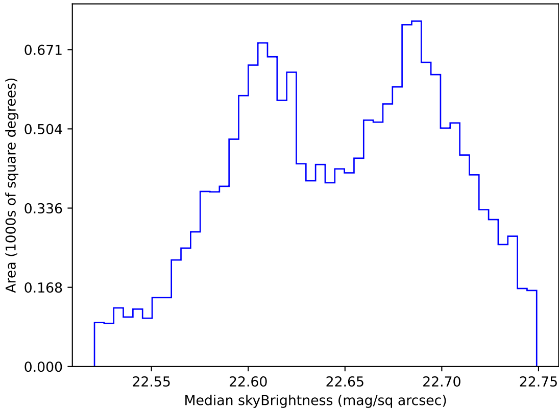
too_elab_r64_d3_griz_v3.4_10yrs WFD u band: Median skyBrightness
