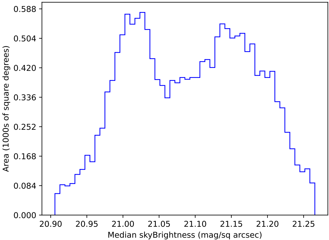
too_elab_r64_d3_griz_v3.4_10yrs WFD r band: Median skyBrightness
