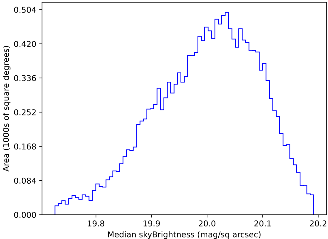
too_elab_r64_d3_griz_v3.4_10yrs WFD i band: Median skyBrightness
