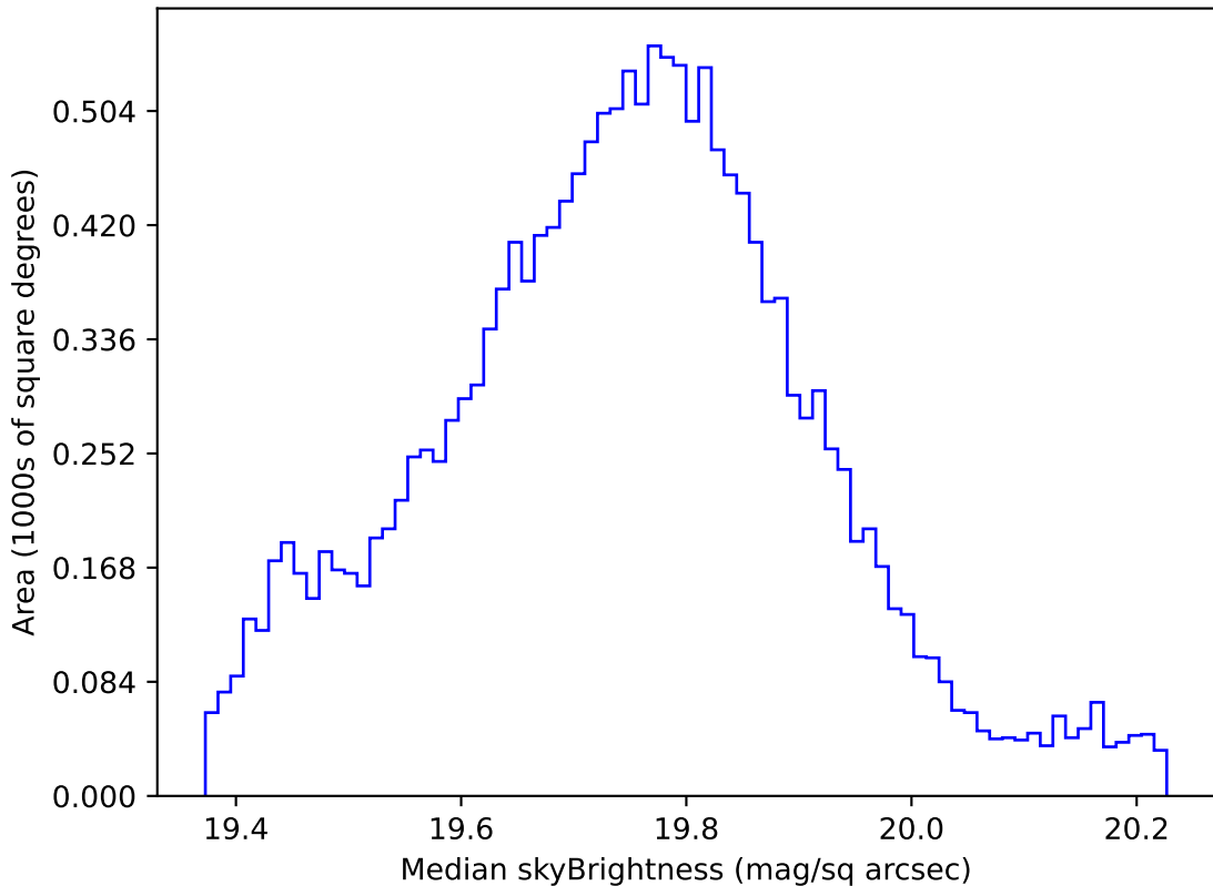
too_elab_r64_d3_griz_v3.4_10yrs WFD all bands: Median skyBrightness
