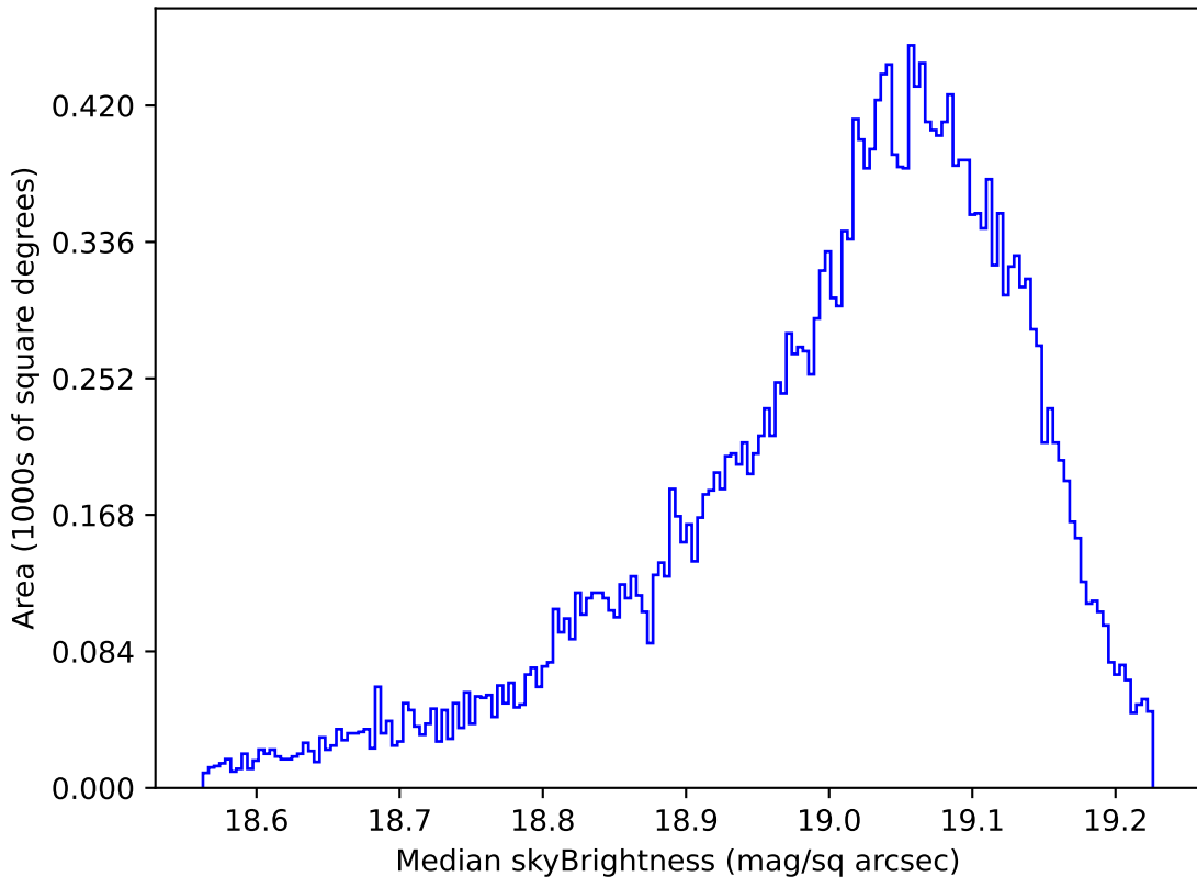
too_elab_r64_d3_griz_v3.4_10yrs All sky z band: Median skyBrightness
