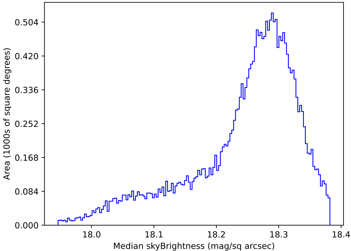
too_elab_r64_d3_griz_v3.4_10yrs All sky y band: Median skyBrightness
