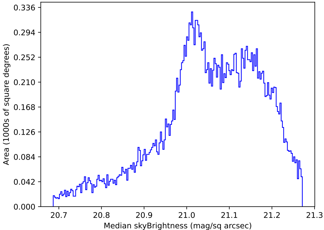
too_elab_r64_d3_griz_v3.4_10yrs All sky r band: Median skyBrightness
