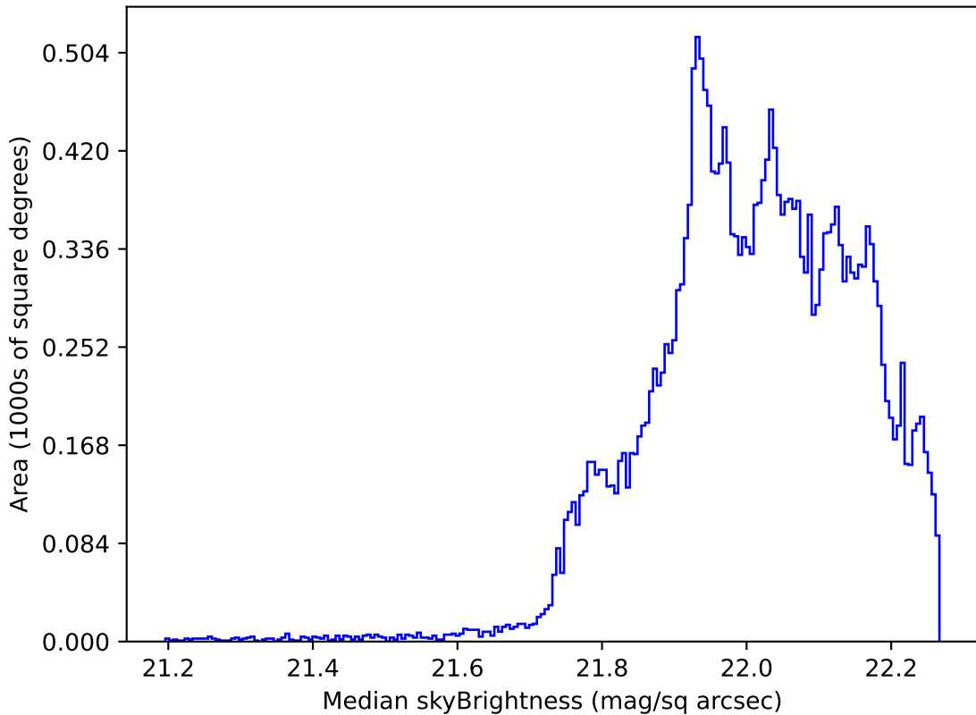
too_elab_r64_d3_griz_v3.4_10yrs All sky g band: Median skyBrightness
