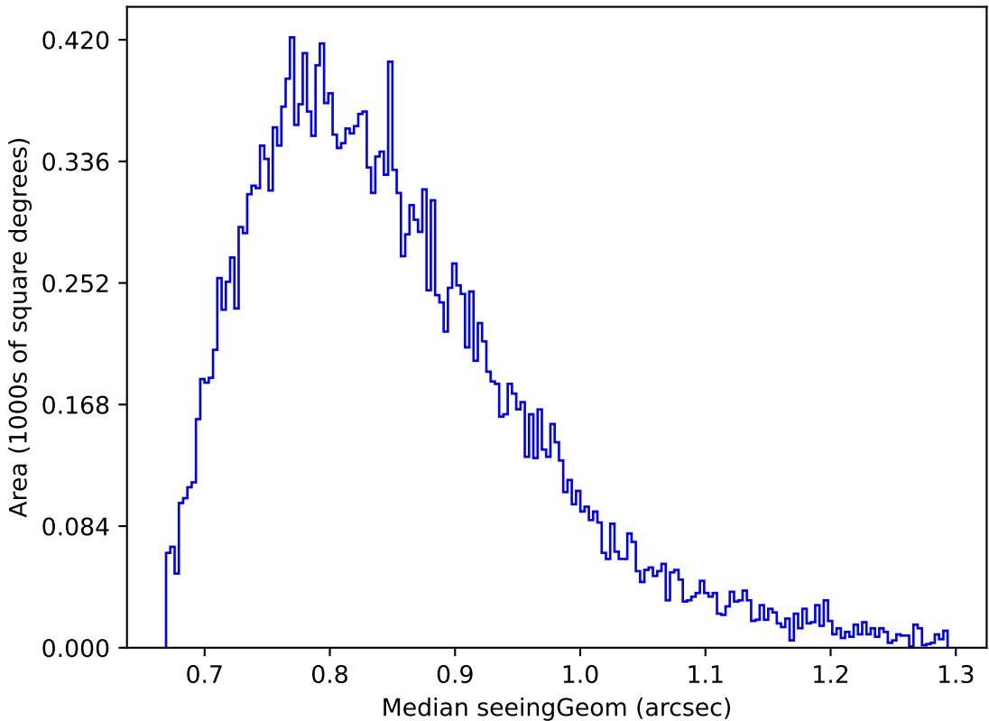
too_elab_r64_d3_griz_v3.4_10yrs Yr 1 z band: Median seeingGeom
