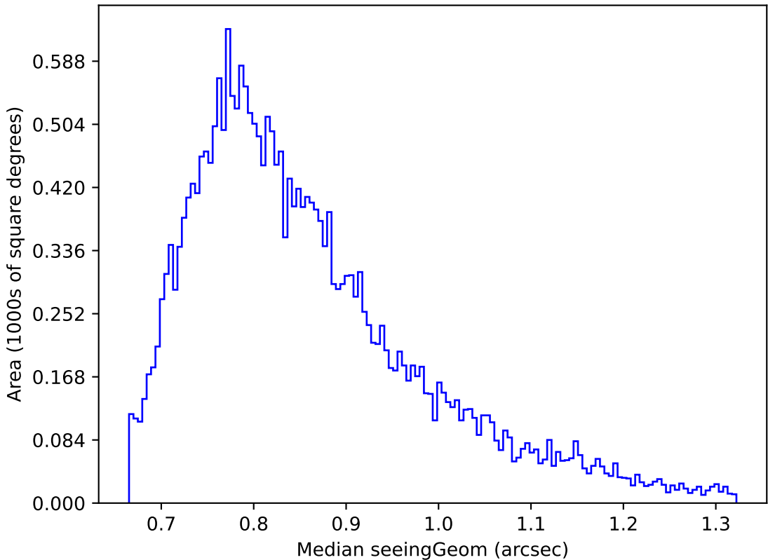
too_elab_r64_d3_griz_v3.4_10yrs Yr 1 r band: Median seeingGeom
