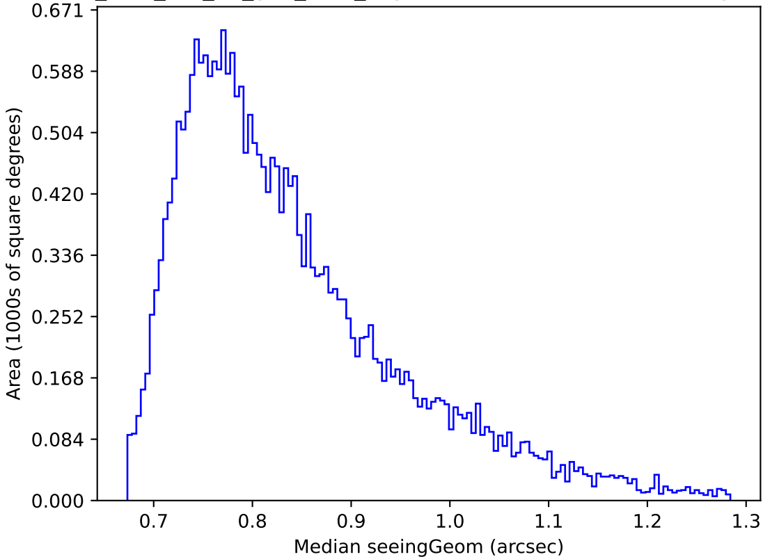
too_elab_r64_d3_griz_v3.4_10yrs Yr 1 i band: Median seeingGeom
