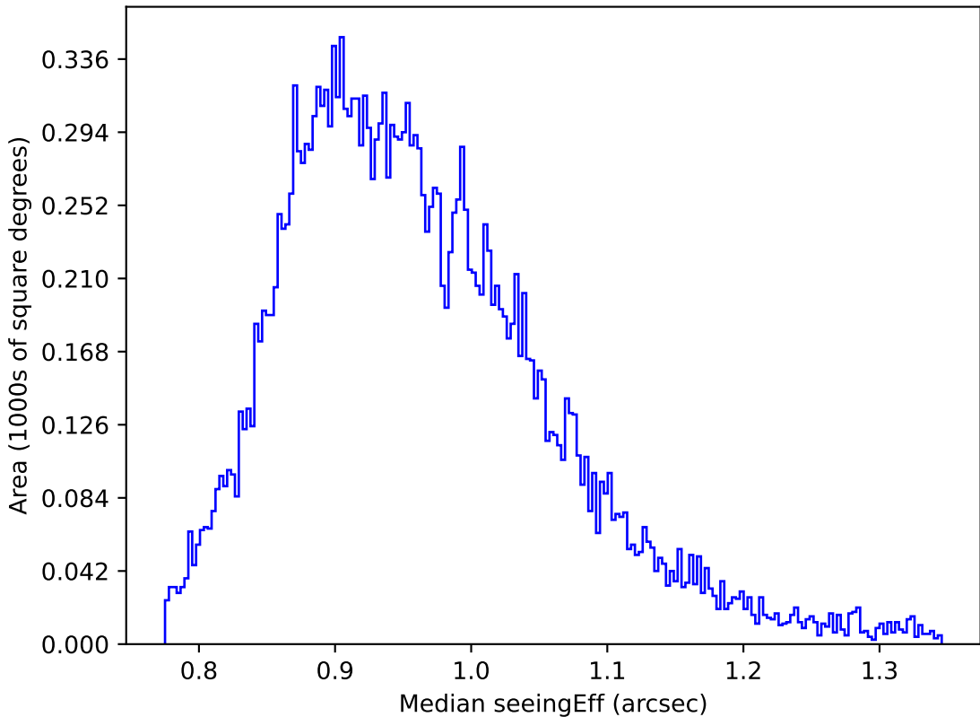
too_elab_r64_d3_griz_v3.4_10yrs Yr 1 y band: Median seeingEff
