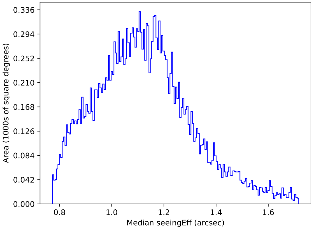
too_elab_r64_d3_griz_v3.4_10yrs Yr 1 u band: Median seeingEff
