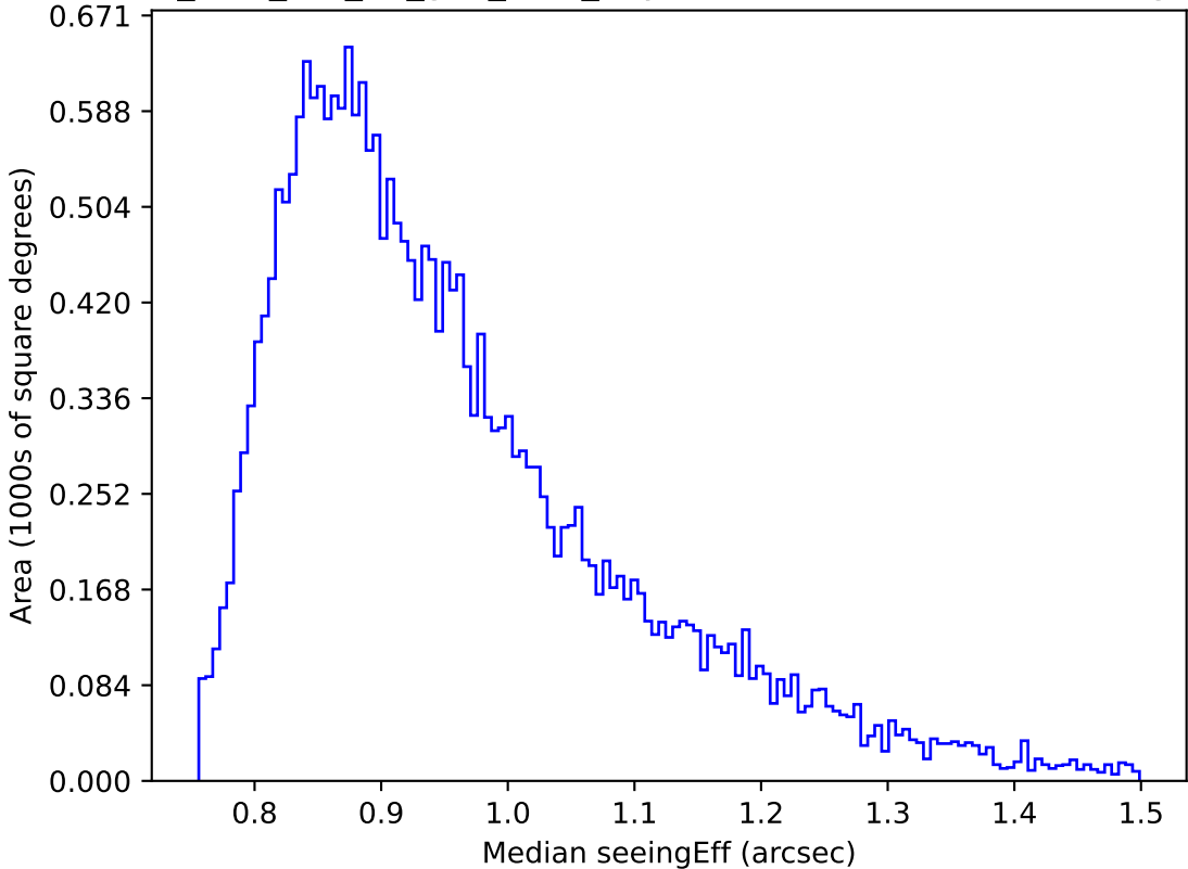
too_elab_r64_d3_griz_v3.4_10yrs Yr 1 i band: Median seeingEff
