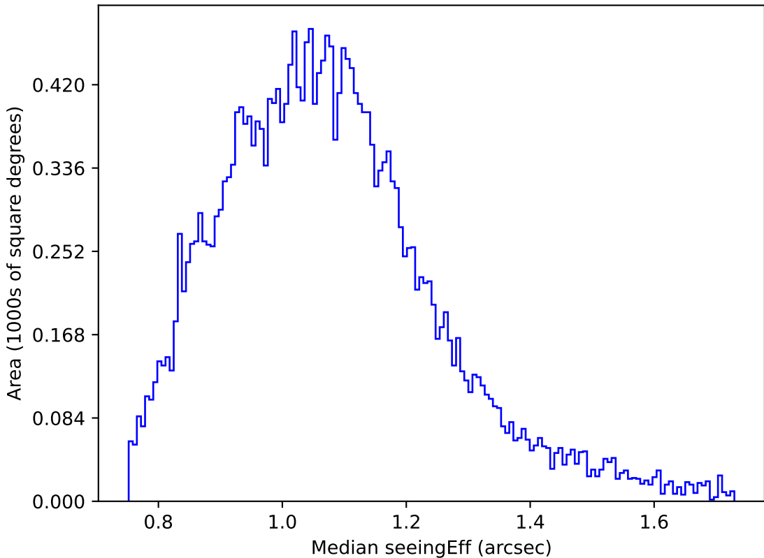
too_elab_r64_d3_griz_v3.4_10yrs Yr 1 g band: Median seeingEff
