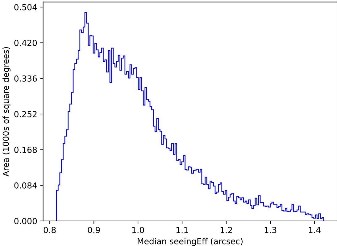
too_elab_r64_d3_griz_v3.4_10yrs Yr 1 all bands: Median seeingEff
