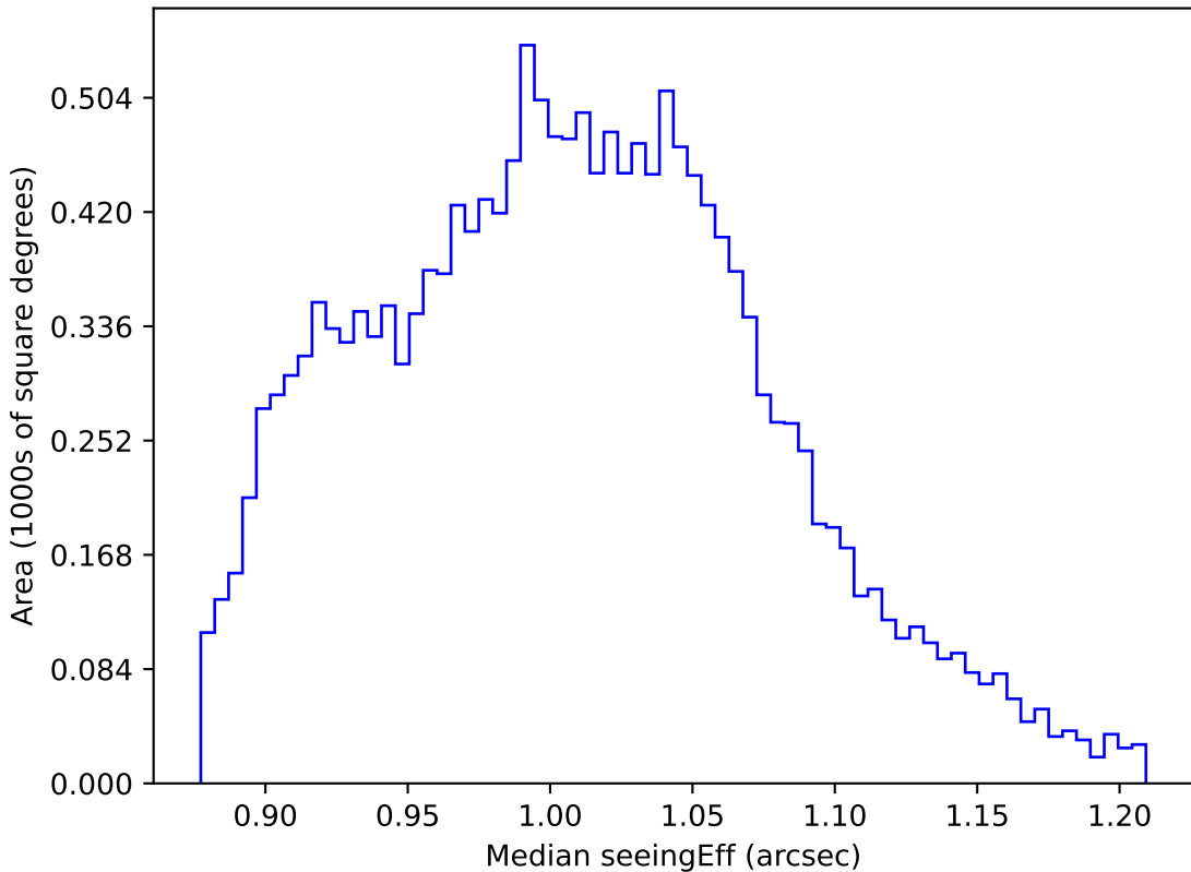
too_elab_r64_d3_griz_v3.4_10yrs WFD z band: Median seeingEff
