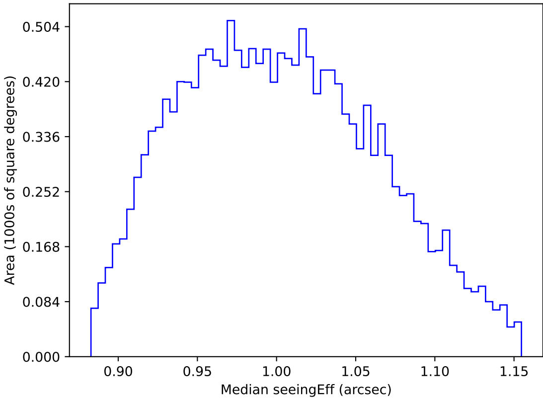
too_elab_r64_d3_griz_v3.4_10yrs WFD y band: Median seeingEff
