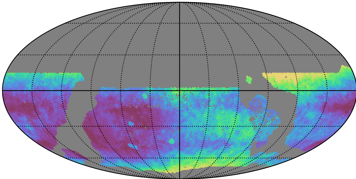
too_elab_r64_d3_griz_v3.4_10yrs WFD r band: Median seeingEff
