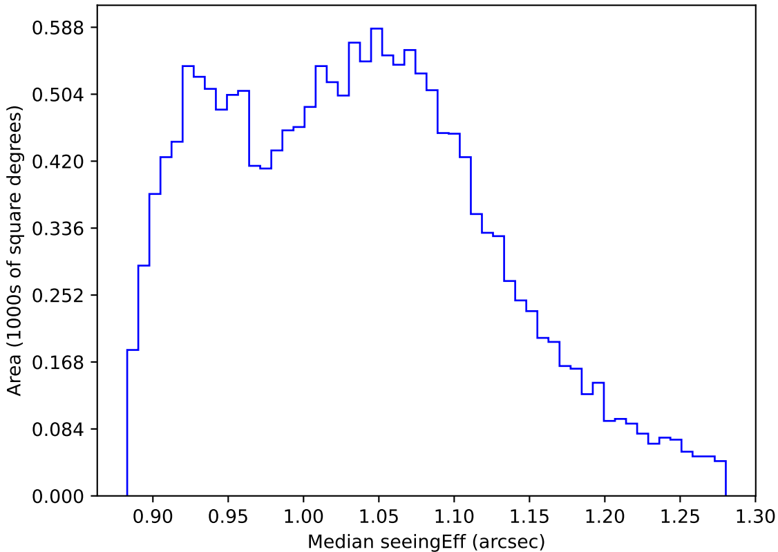
too_elab_r64_d3_griz_v3.4_10yrs WFD r band: Median seeingEff
