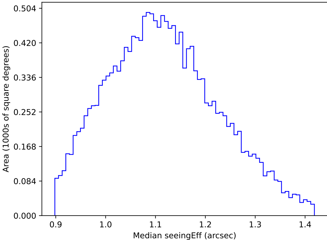
too_elab_r64_d3_griz_v3.4_10yrs WFD g band: Median seeingEff
