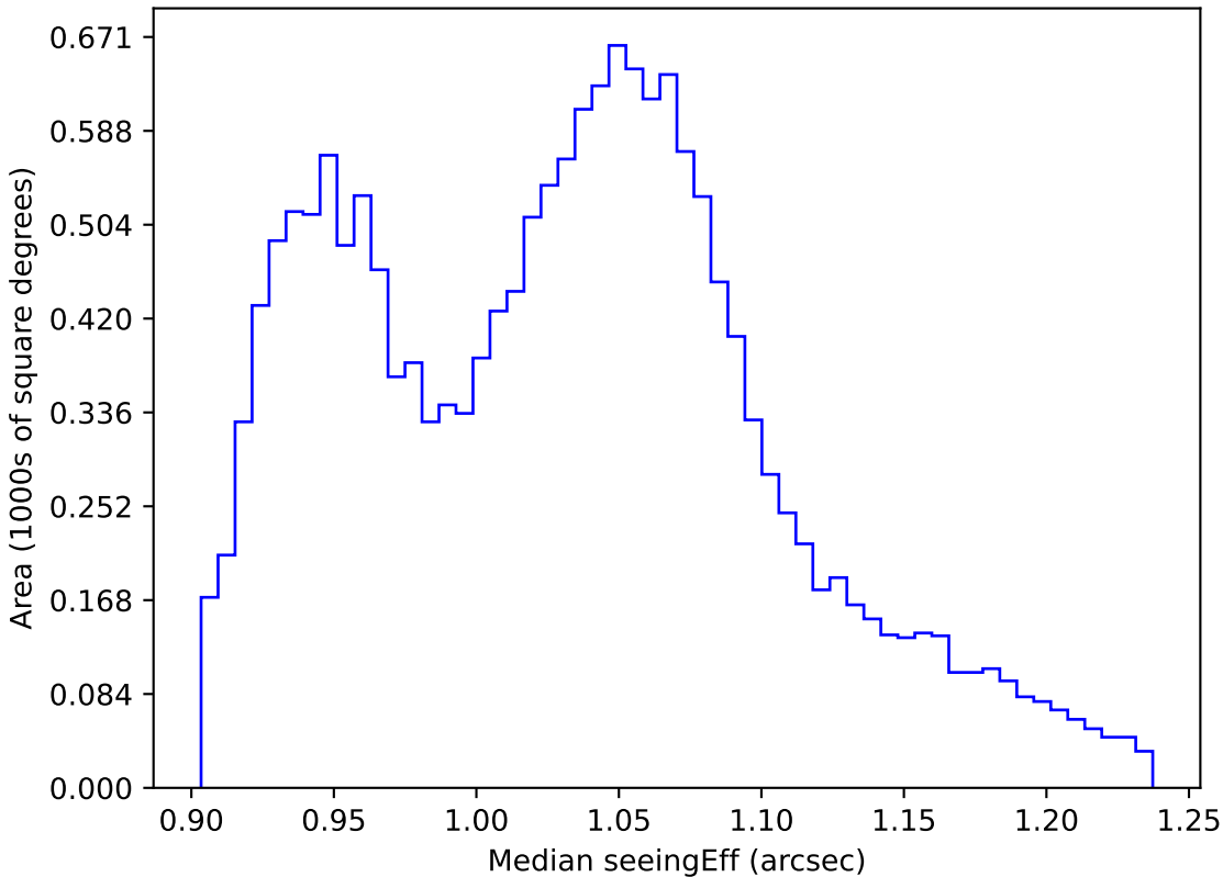
too_elab_r64_d3_griz_v3.4_10yrs WFD all bands: Median seeingEff
