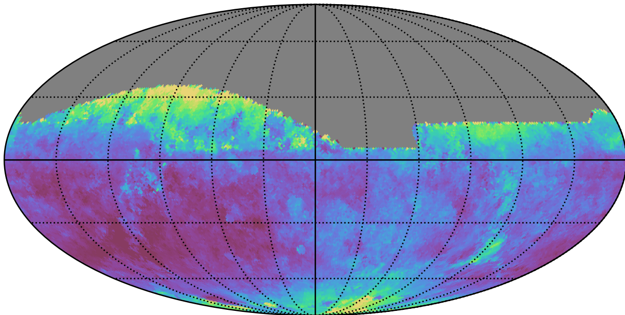
too_elab_r64_d3_griz_v3.4_10yrs All sky z band: Median seeingEff
