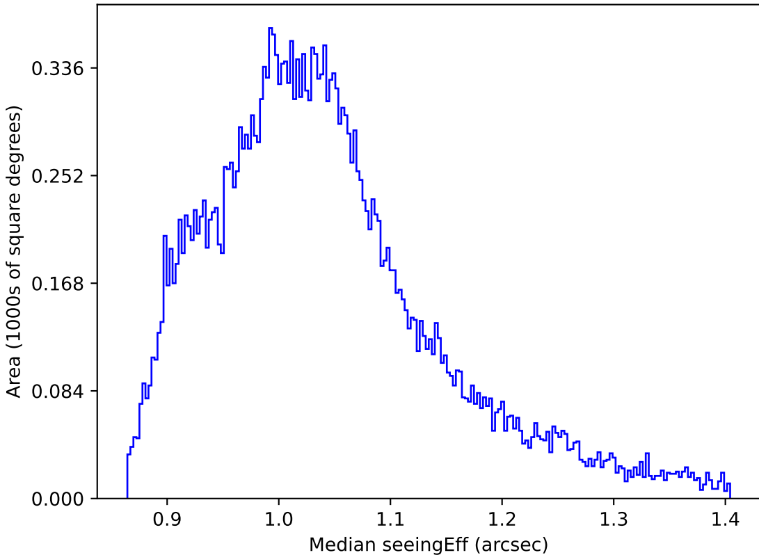
too_elab_r64_d3_griz_v3.4_10yrs All sky z band: Median seeingEff
