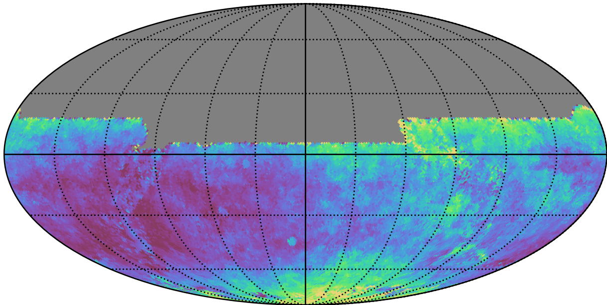
too_elab_r64_d3_griz_v3.4_10yrs All sky y band: Median seeingEff
