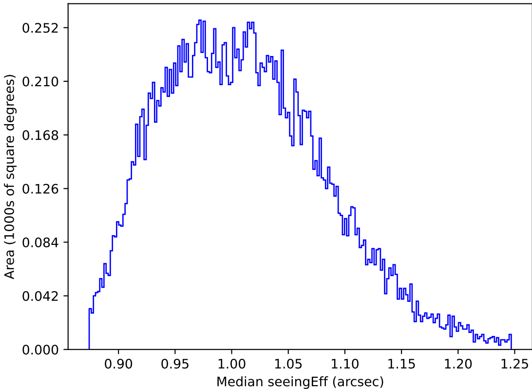
too_elab_r64_d3_griz_v3.4_10yrs All sky y band: Median seeingEff
