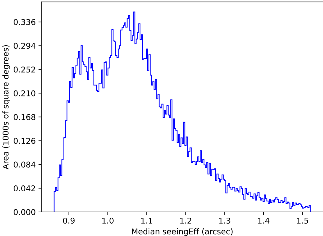
too_elab_r64_d3_griz_v3.4_10yrs All sky r band: Median seeingEff
