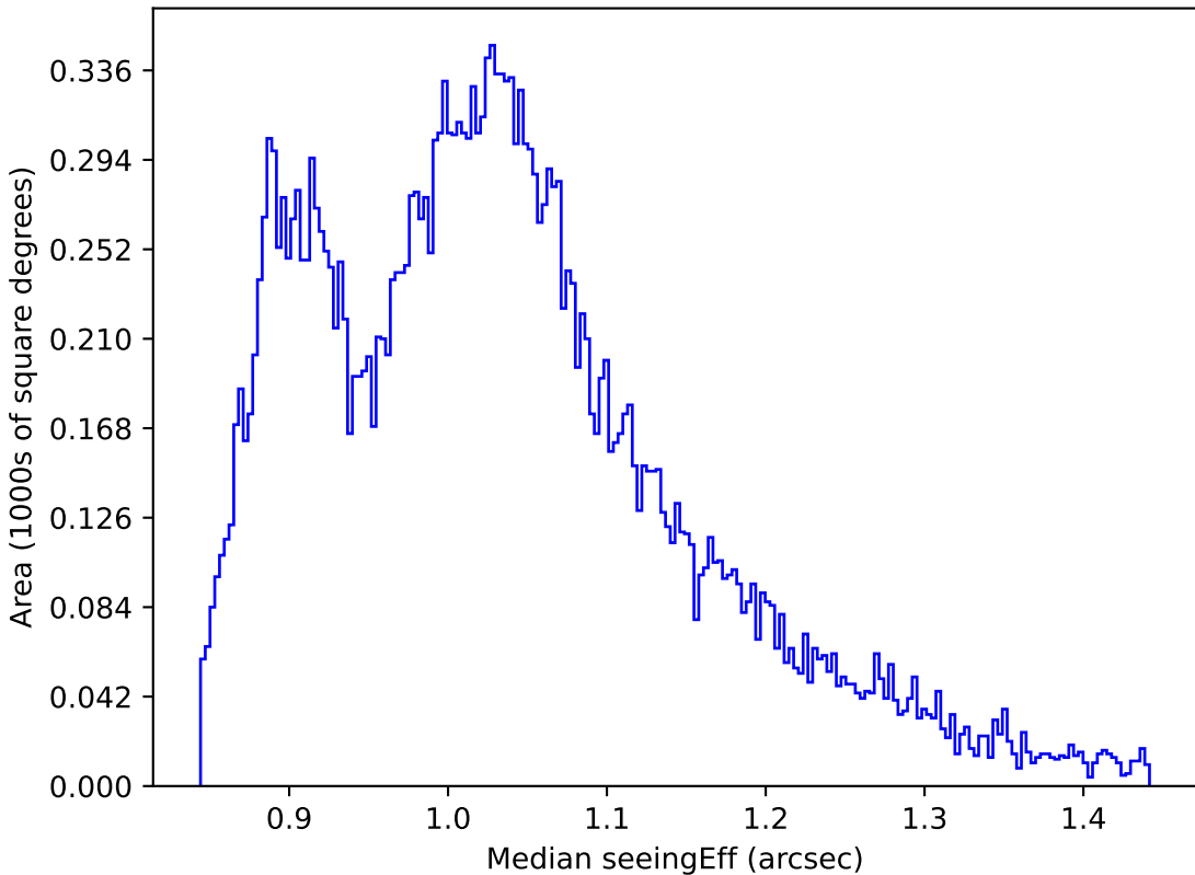
too_elab_r64_d3_griz_v3.4_10yrs All sky i band: Median seeingEff
