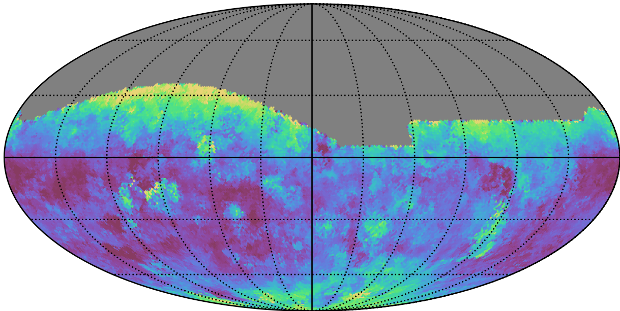
too_elab_r64_d3_griz_v3.4_10yrs All sky g band: Median seeingEff
