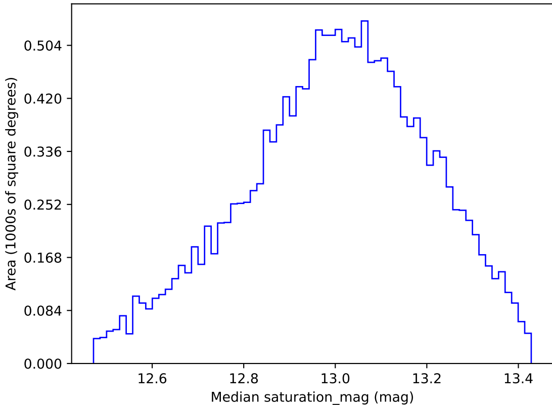
too_elab_r64_d3_griz_v3.4_10yrs WFD u band: Median saturation_mag
