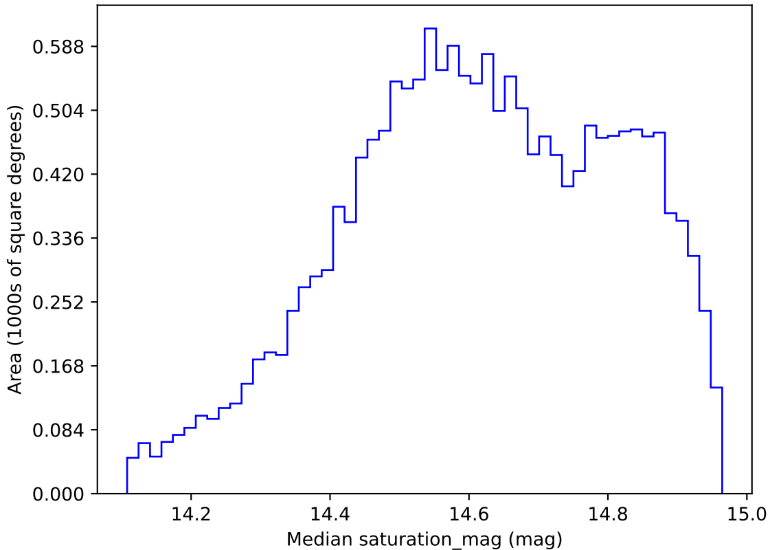
too_elab_r64_d3_griz_v3.4_10yrs WFD r band: Median saturation_mag
