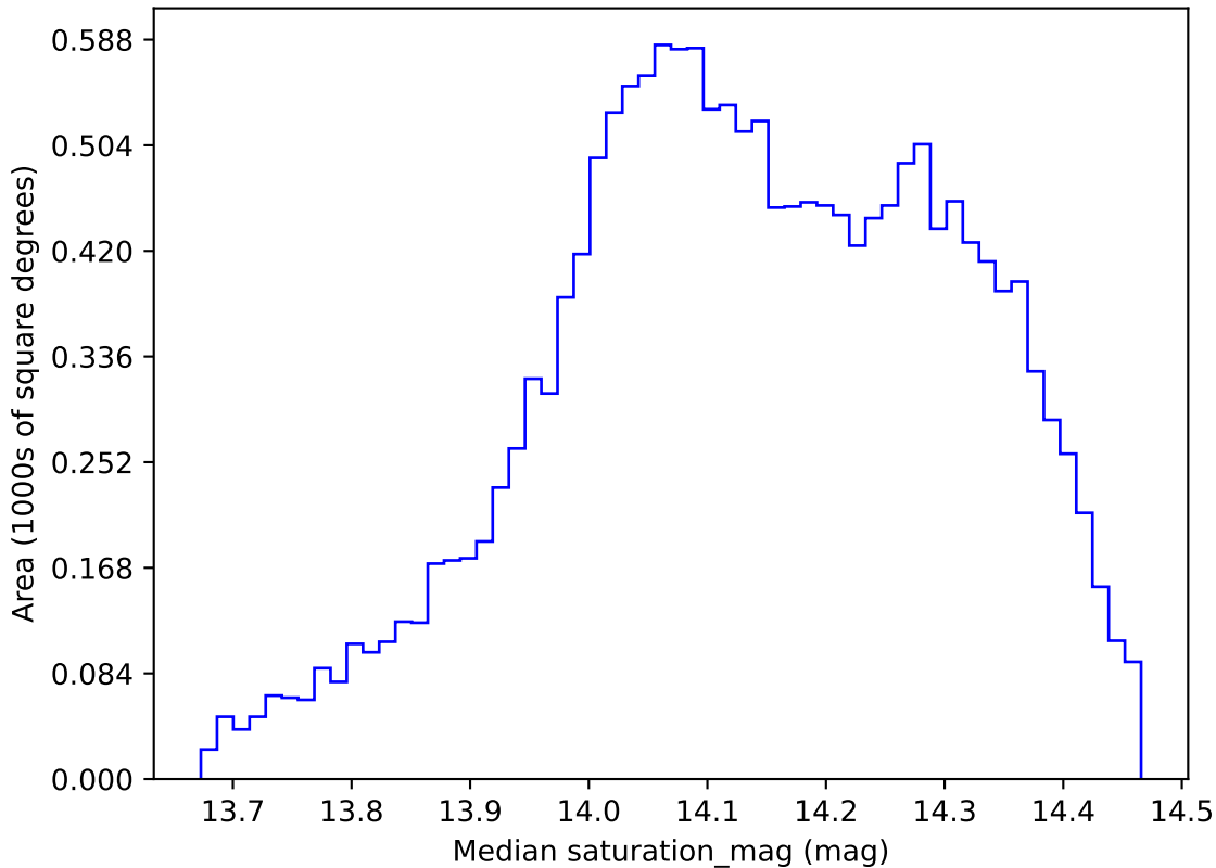
too_elab_r64_d3_griz_v3.4_10yrs WFD all bands: Median saturation_mag
